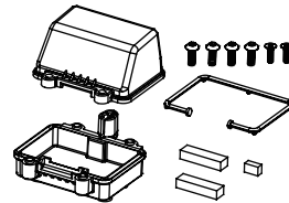
FTX11008 receiver box 1set
